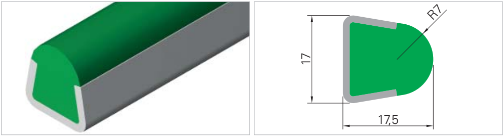
RP CI S 01 (stainless steel material: AISI 304)
