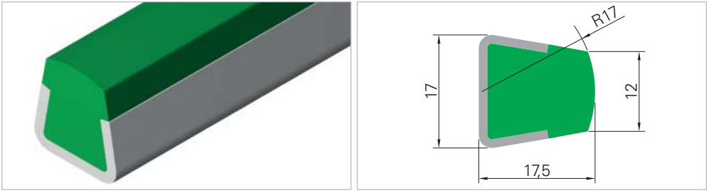
RP CI S 02 (stainless steel material: AISI 304)
