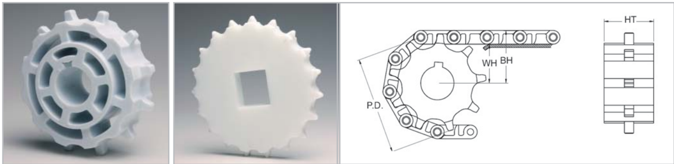
Molded sprocket
