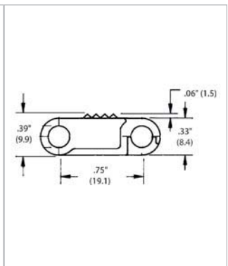
Rough Top
