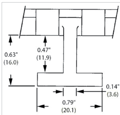
Hold-down tabs
