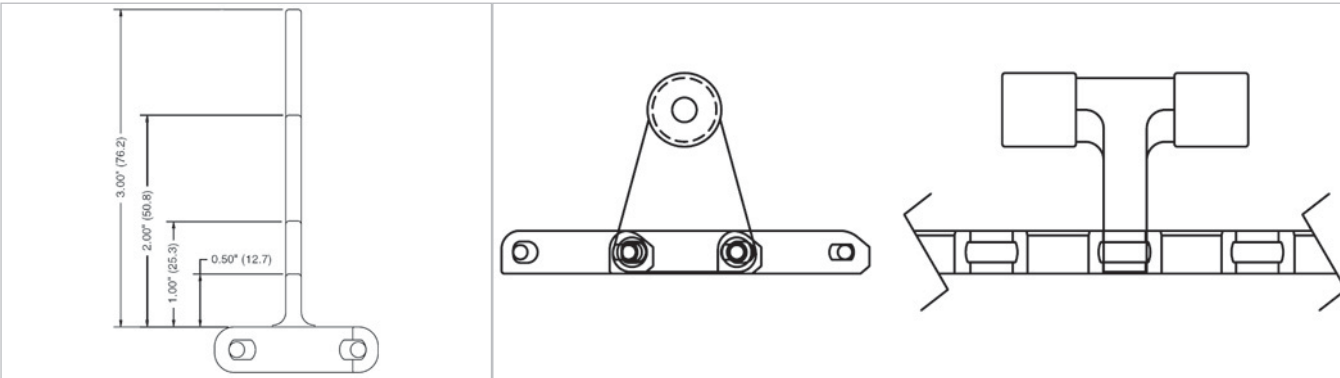
Flights Standard flights are available in 1/2", 1", 2" and 3" heights
