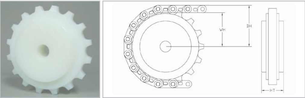
Machined sprocket
